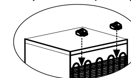
Rear stoppers (installation by owner)
