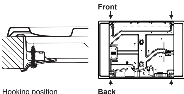
Hooking position for top H=40mm
